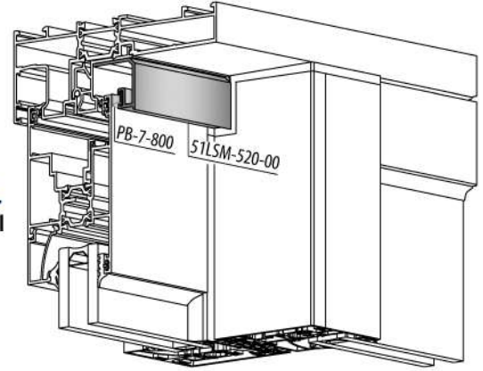
B DETAIL DETAYI
