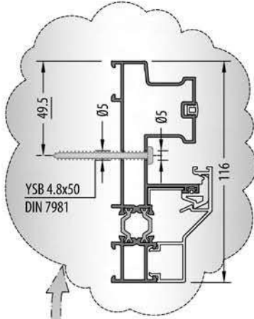
B DETAIL DETAYI
