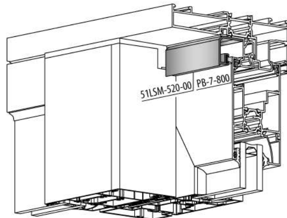
C DETAIL DETAYI
