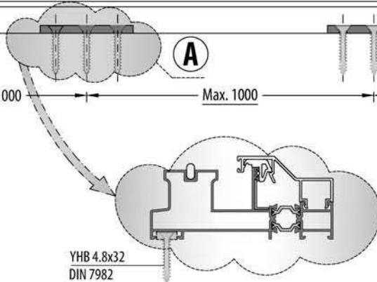
A DETAIL DETAYI
