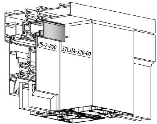
D DETAIL DETAYI
