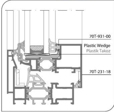
SECTION / KESİT
