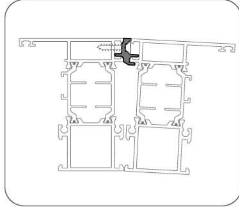
APPLICATION DETAIL / UYGULAMA DETAYI
